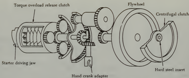
FIGURE 5-1. Combination hand and electric inertia starter.
